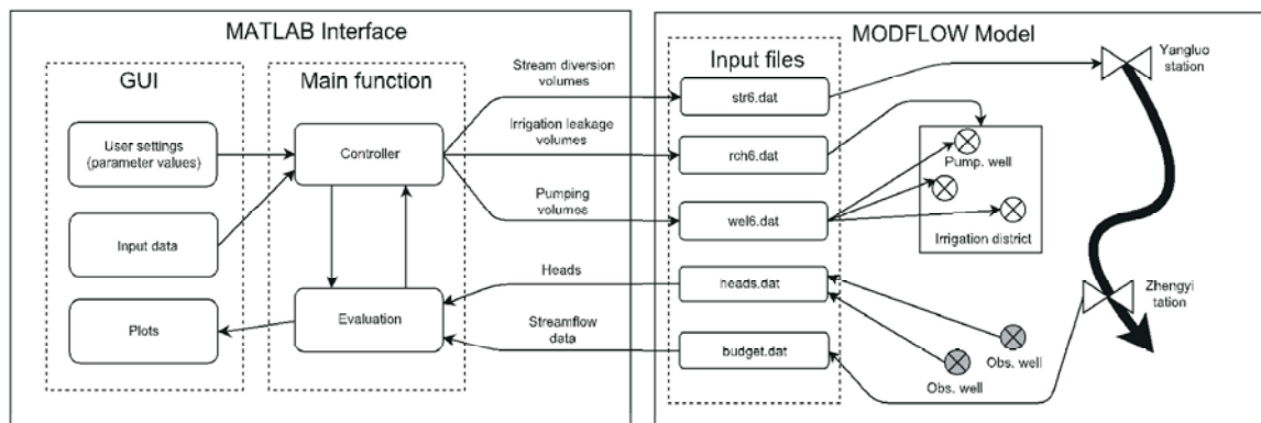
Fig. 8: Coupling of optimization module to groundwater/surface water model
