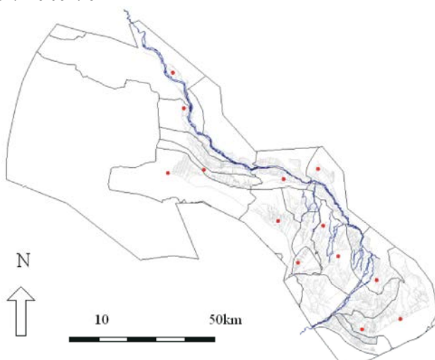
Fig. 7: Irrigation water supply system of the Heihe mid-reach consisting of surface irrigation canals and pumping wells organized in 20 irrigation districts. The red points indicate the locations of the observation wells selected for the computation of the head indicator
