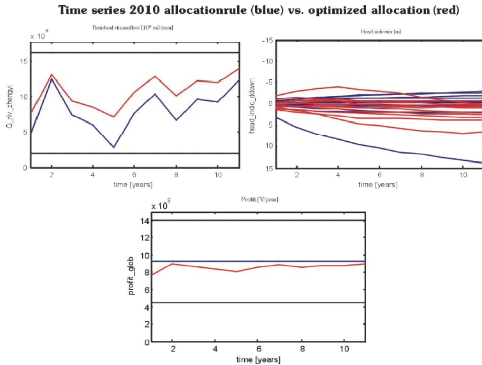
Fig. 11: Results of optimal control over a period of 10 years: Development of profits, residual flows to downstream and groundwater heads (heads shown for all control points)
