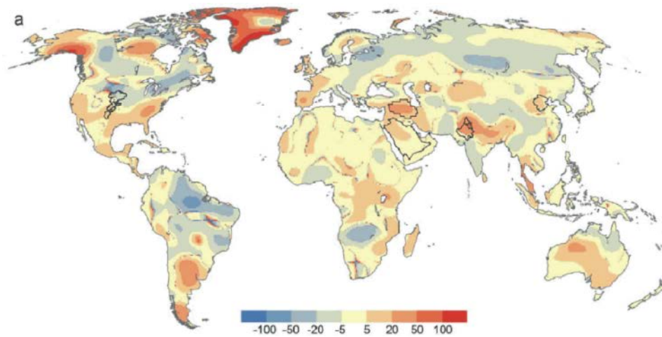
Fig. 2: Change in water storage 2003 to 2009 as observed by GRACE (average of 3 interpretations) [5] (Units: mm/yr, blue increase, red decrease of storage)
