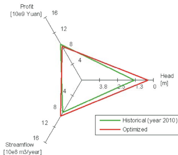
Fig. 9: Spider plot for the year 2010 comparing current allocation with the theoretically optimal allocation.
