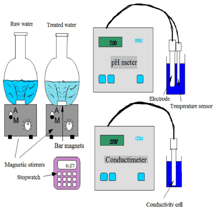
Fig. 1: Experimental apparatus used in the process of rapid controlled precipitation
